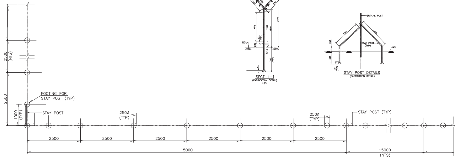
PLAN OF FOUNDATION
