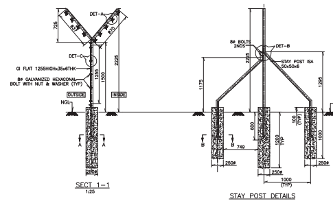
STAY POST DETAILS 1:25
