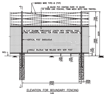
ELEVATION FOR BOUNDARY FENCING 1:25
